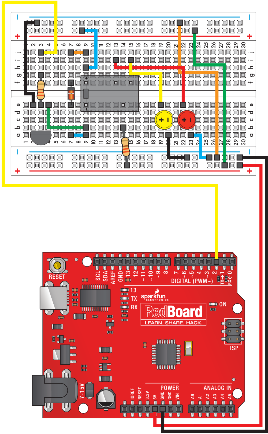
Circuit 13: Relays
